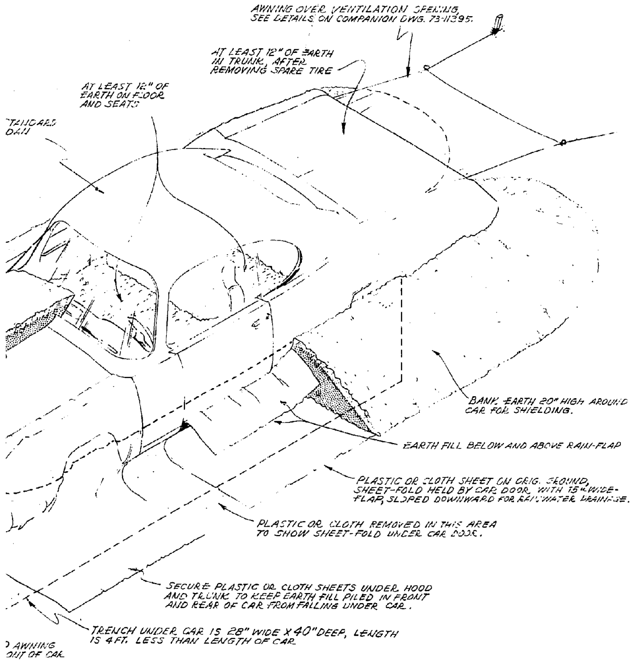
13.1. Car-Over-Trench Shelter, Pictorial View.
